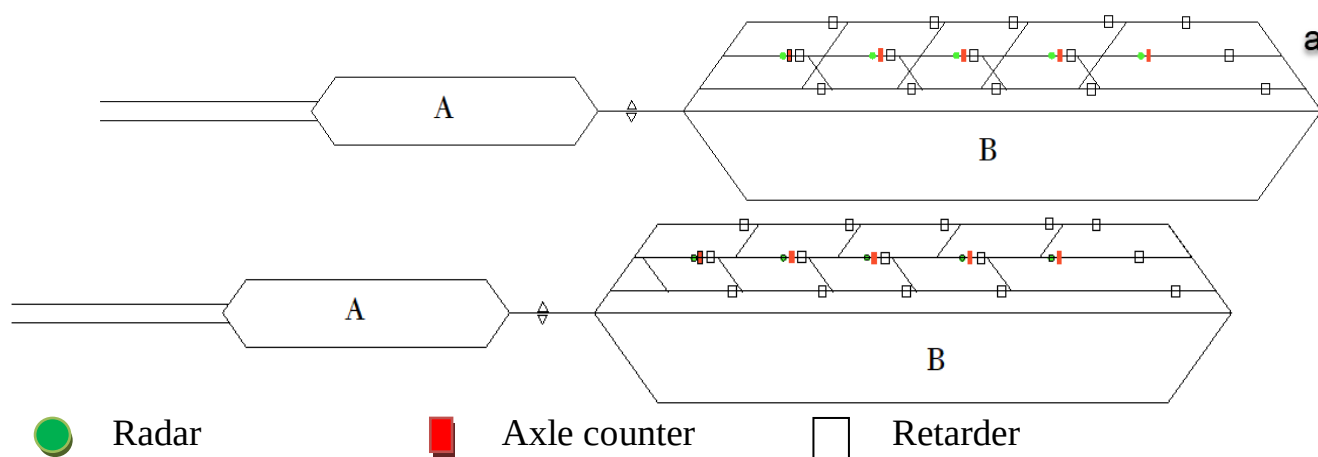
Figure 1. Technical solutions for forming feeder trains by Japanese method: a) with simple crossovers; b) with double crossovers
