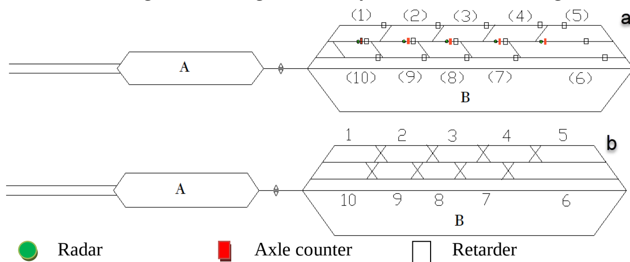
Figure 2. Track use during feeder train forming by Japanese method a) for solution with simple crossovers; b) for solution with double crossovers
